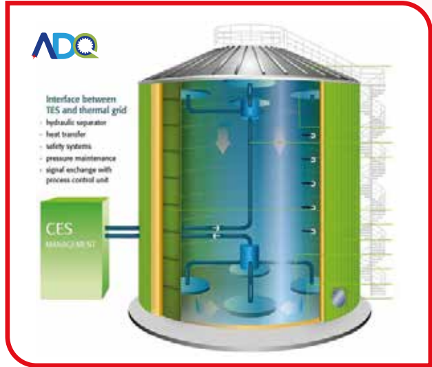
THERMAL ENERGY STORAGE TANK
